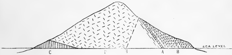
Fig. 1.—Sketch section through Yacaaba Headland. A, Limestone with associated Tuffs; B, Conglomerates; C, Andesite; D, Toscanite. H, Fault.
